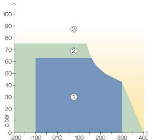
pT diagram for thickness 2.0 mm
